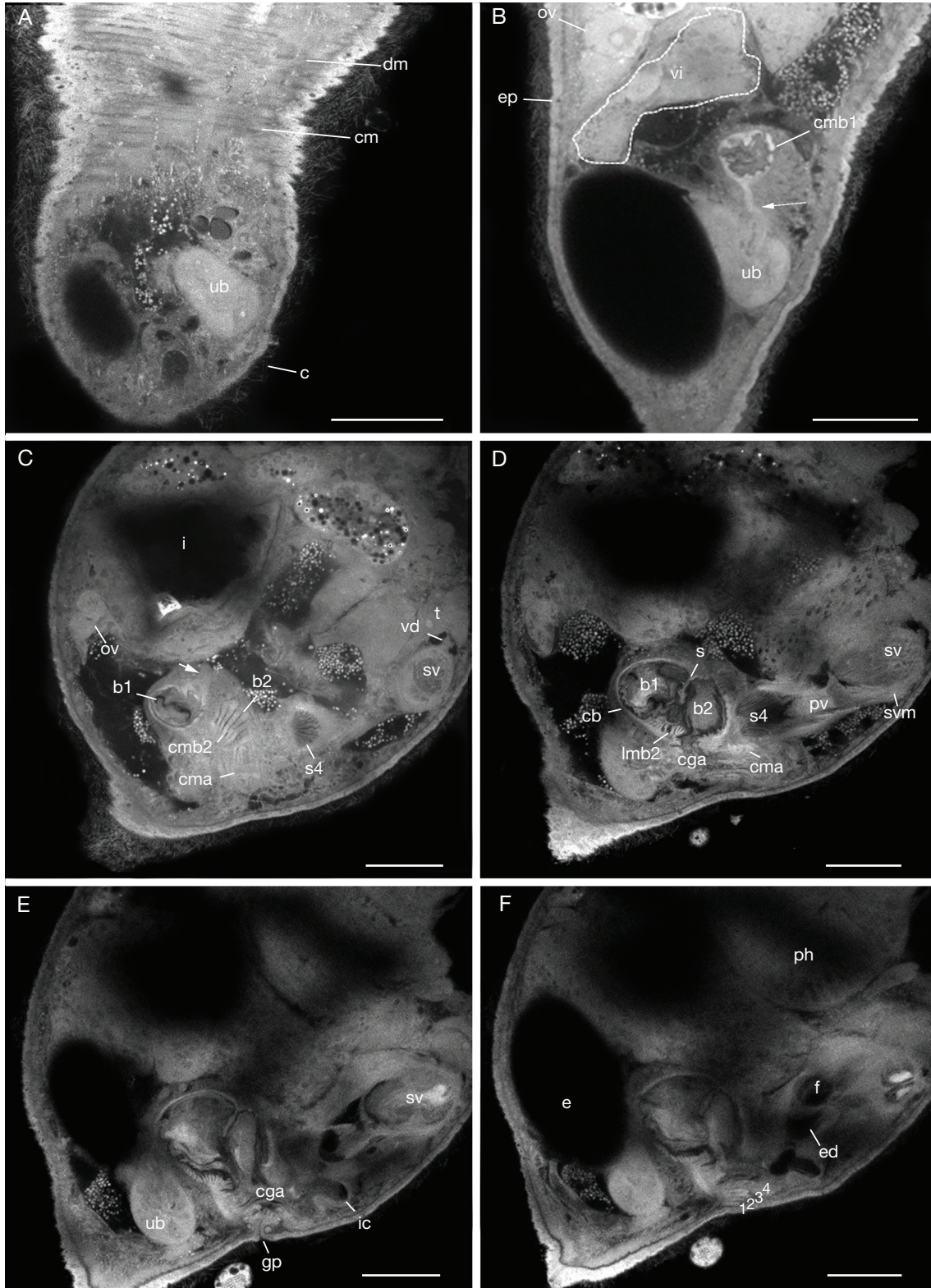
FIG. 3. — Giaysztoria reta n. sp. CLSM images of whole-mounts labeled with rhodamine-phalloidin showing the muscle arrangement: A, B , caudal body section from dorsal to ventral plane; C-F , caudal body section viewed from the right side toward the left side to sagittal plane. Images A, B and C-F correspond to two different specimens. Numbers 1-4 indicate circular fibers of gonopore sphincter; dashed lines outline the vitellaria area. Continuous arrow indicates strong muscle fiber of bursa cavity. Dashed arrow indicates muscle fiber that associates the uterus bend with the copulatory bursa. Abbreviations: b1 , copulatory bursa cavity 1; b2 , copulatory bursa cavity 2; c , cilia; cb , copulatory bursa; cga , common genital atrium; cm , circular muscle fibers of the body wall; cma , circular muscle fibers of common genital atrium; cmb1 , circular muscles of the bursa cavity 1; cmb2 , circular muscles of bursa cavity 2; dm , diagonal muscle fibers of the body wall; e , egg; ed , ejaculatory duct; ep , epidermis; gp , gonopore; i , intestine; ic , insertion cavity of s1 spine; ov , ovary; ph , pharynx; pv , prostate vesicle; s , septum; sv , seminal vesicle; svm , muscular wall of seminal vesicle; s4 , group of dorsal hollow spines; t , testes; ub , uterus bend; vd , vasa deferentia; vi , vitellaria. Scale bars: A, B, 50 µm; C, D, E, F 40 µm.
