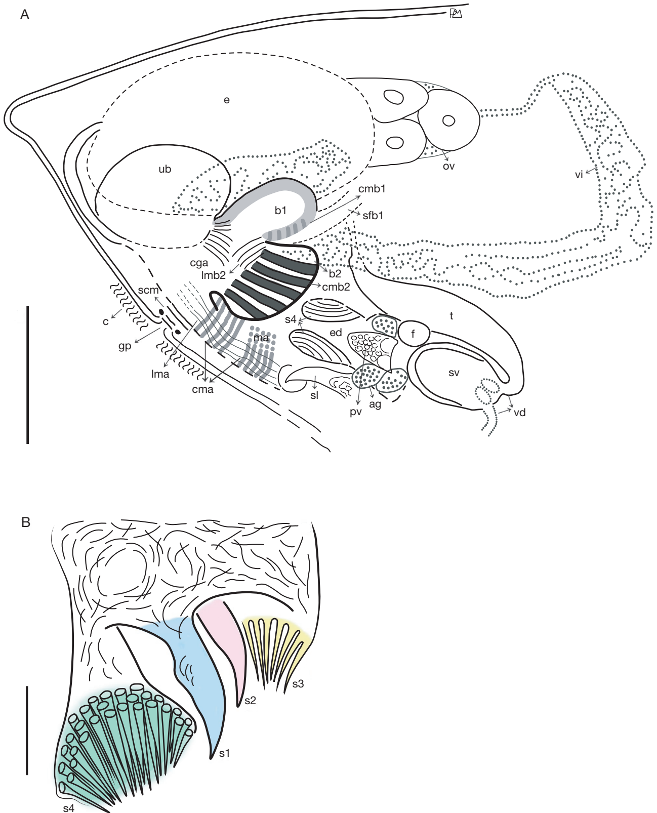
FIG. 4. — Graphic reconstruction of the genital system of Gieysztorita reta n. sp.: A , genital reconstruction using confocal microscopy images; B , penis stylet from the holotype, blue ( s1 ), pink ( s2 ), yellow ( s3 ) and green ( s4 ). Abbreviations: ag , accessory glands; b1 , copulatory bursa cavity 1; b2 , copulatory bursa cavity 2; c , cilia; cga , common genital atrium; cma , circular muscle fibers of common genital atrium; cmb1 , circular muscles of the bursa cavity 1; cmb2 , circular muscles of bursa cavity 2; e , egg; ed , ejaculatory duct; f , fenestra; gp , gonopore; ma , male genital atrium; lma , longitudinal muscles fibers of common genital atrium; lmb2 , longitudinal muscle of bursa cavity 2; ov , ovary; pv , prostate vesicle; sfb1 , strong muscle fiber of bursa cavity 1; scm , muscle fibers of gonopore sphincter; sv , seminal vesicle; s1 , largest spine; s2 , large spine; s3 , group of fine short spines; s4 , group of hollow spines; t , testes; ub , uterus bend; vd , vasa deferentia; vi , vitellaria. Scale bars: A, 50 \mu m; B, 20 \mu m.
