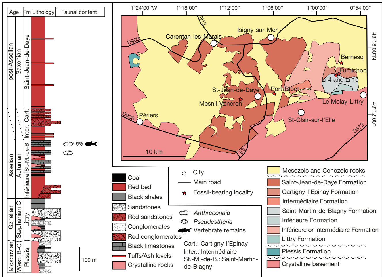
Fig. 2. — Geological map and stratigraphy of the Carentan Basin (modified after L'Homér & Pareyn 1989). Schema and map by D. Gonçalves.
