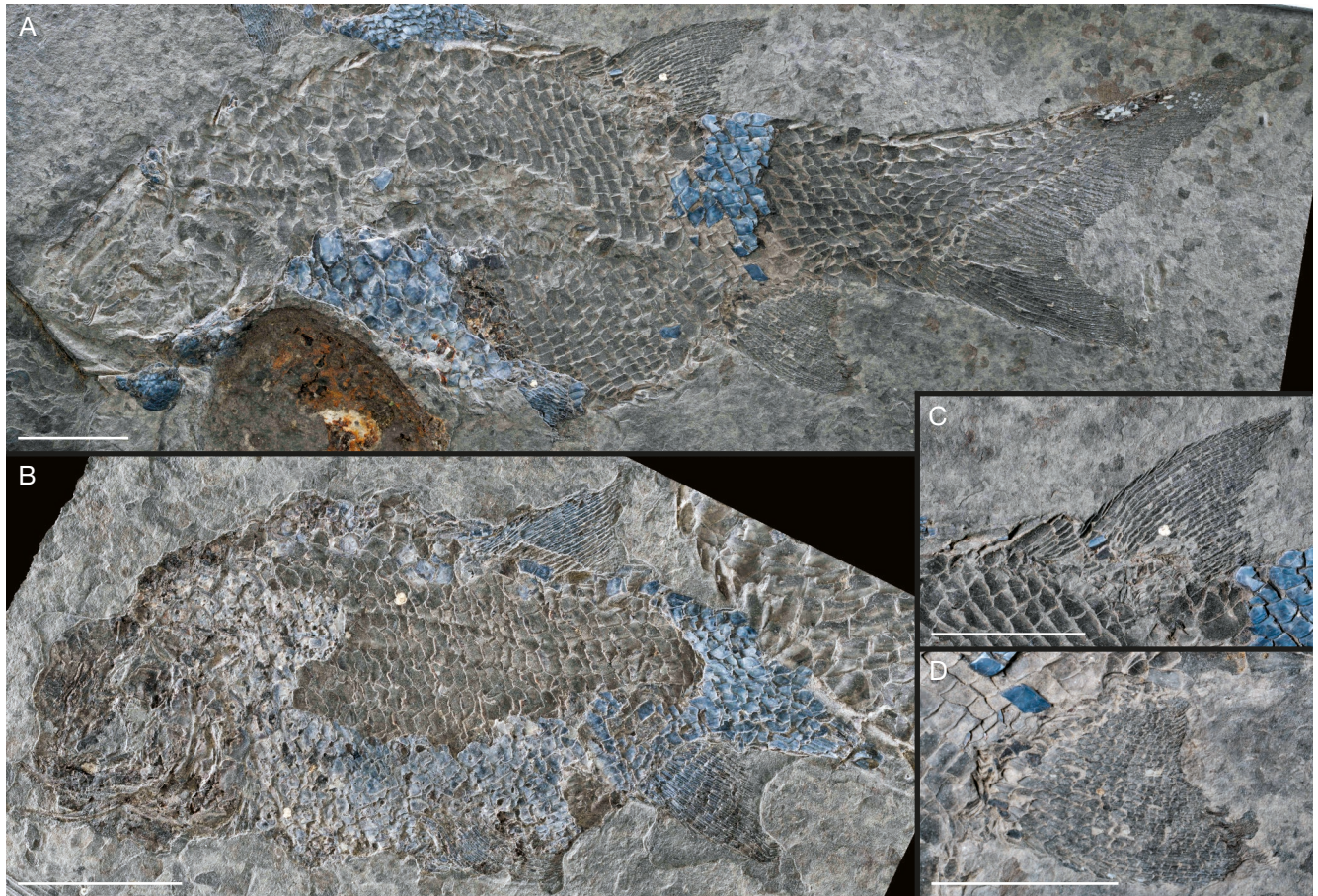
FIG. 7. — Aeduellina blainvillei (Agassiz, 1833) from the Stephanian C of Les Effretais, Saint-Pierre-la-Cour Basin: A , ML-PAL-0451a; B , ML-PAL-0451b, reverted; C , detail of the dorsal fin of ML-PAL-0451a; D , detail of the anal fin of ML-PAL-0451a. Scale bars: 1 cm. Photos: ML, modified by D. Gonçalves.
