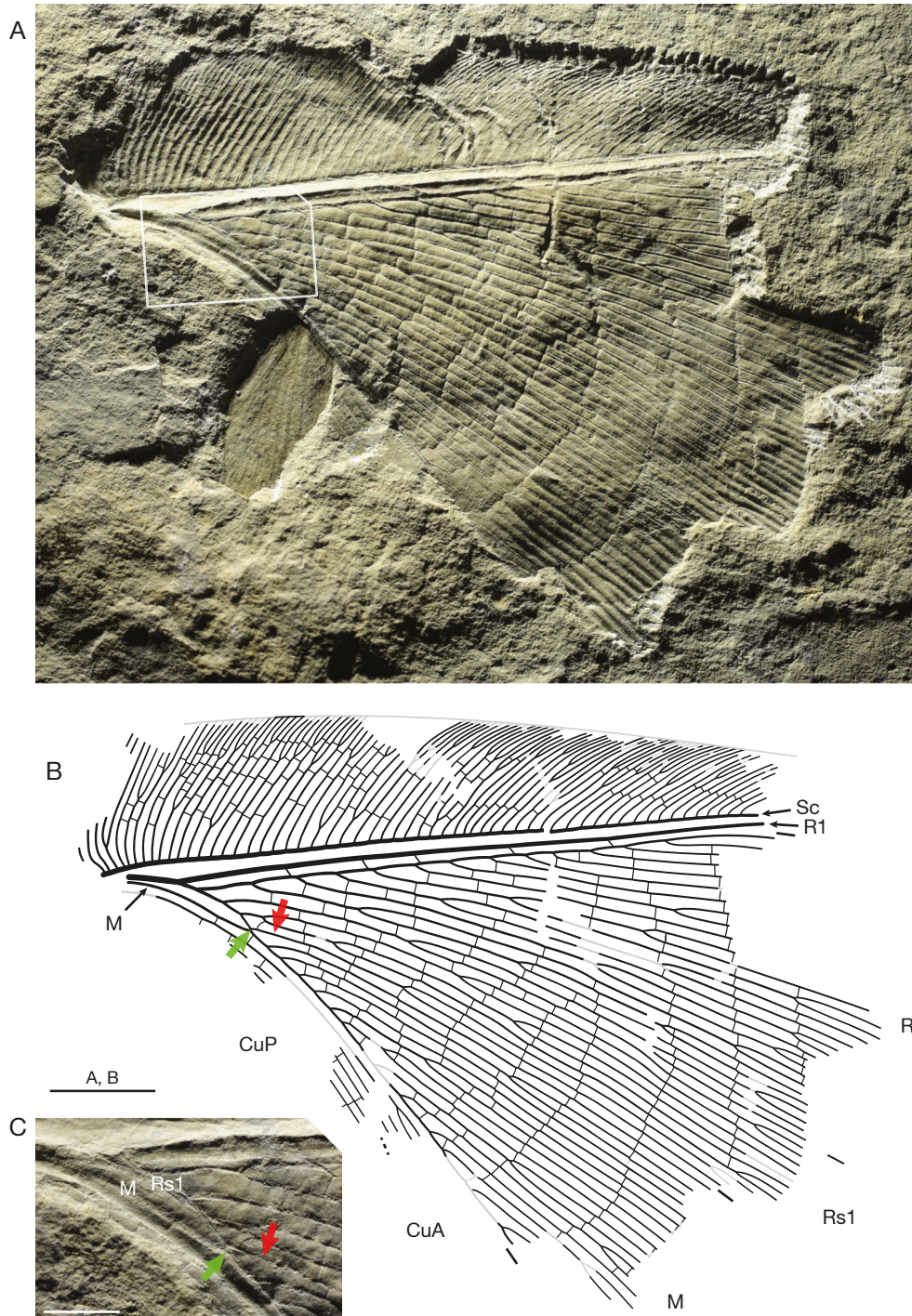
FIG. 1. — Moltenopsychops magnus n. gen., n. sp. (Osmylopsychopidae), holotype PRE/F/21985, right forewing (Moltano Formation; Upper Triassic; South Africa): A, B , overview; A , photograph (positive imprint); B , interpretative drawing (green arrow, rs_1 -m cross-vein; red arrow, Rs_1 posterior-most branch); C , detail of the rs_1 -m cross-vein and surrounding structures, photograph (positive imprint; location as shown on A ; large arrows, as in B ). Scale bars: A, B, 5 mm; C, 2 mm. Photographs and drawing: O. Béthoux.
