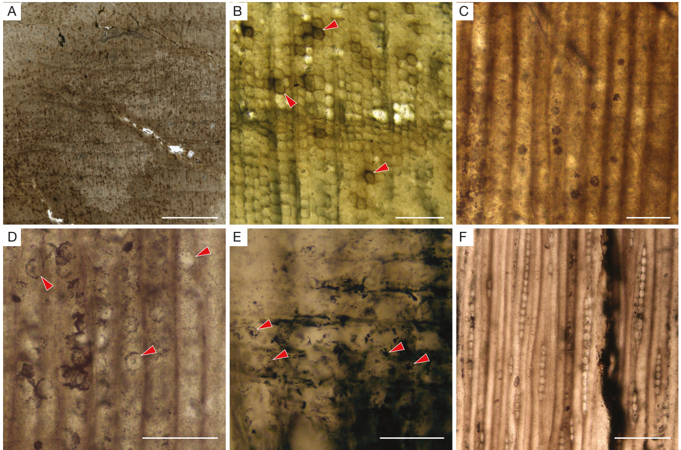
FIG. 5. — Indeterminate abietinean type, MPEF-Pb 10663 (A, B, D-F) and MPEF-Pb 10673 (C): A, poorly distinct growth ring boundaries (TS); B, tracheids with circular to polygonal sections (TS). Note some isolated tracheids with thicker walls and darker lumens (arrowheads); C, D, abietinean radial pitting (RLS); E, cross-fields with bordered pits (arrowheads) (RLS). Note the poorly preserved pits (arrowheads); F, uniseriate rays (TLS). Scale bars: A, 3 mm; B, 200 \mu m; C, D, 100 \mu m; E, 50 \mu m; F, 200 \mu m. Photos: Carlos Daniel Greppi.
