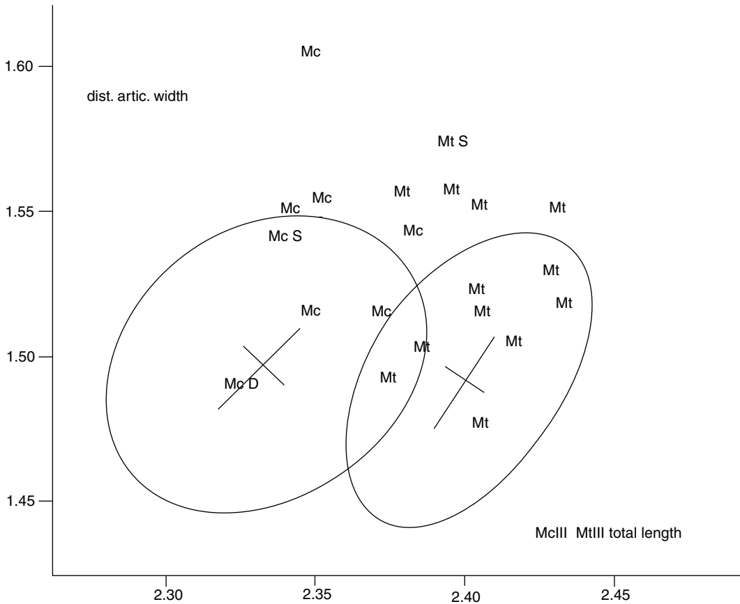
FIG. 3. — Distal articular breadth plotted to total length in Mc and MtIII of hipparions of the H. mediterraneum group; log data of measurements in mm. 95% equiprobability ellipses drawn on the hypodigm sample of H. mediterraneum from Pikermi. Plotted are specimens from Darayaspoon ( Mc D ), Sor ( Mc , Mt S ) and Bazaleti ( Mc , Mt without locality abbreviation).
