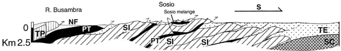
FIG. 2. — Interpretative geologic section across the Rocca Busambra-Sicani Mountains area based on surface data (location in Fig. 1): TP, Trapanese units (Late Triassic-Miocene); NF, Numidian Flysch units (Late Oligocene-Early Miocene); SI, Sicanian units (Late Triassic-Early Tertiary); PT, Permian-Carnian units; SC, Saccense units (Late Triassic-Miocene); TE, Oligo-Miocene, mostly terrigenous, deformed covers. The thick allochthon of Permian-Carnian deposits dipping below the Rocca Busambra Unit represent the westward extension of the Lercara structure.
