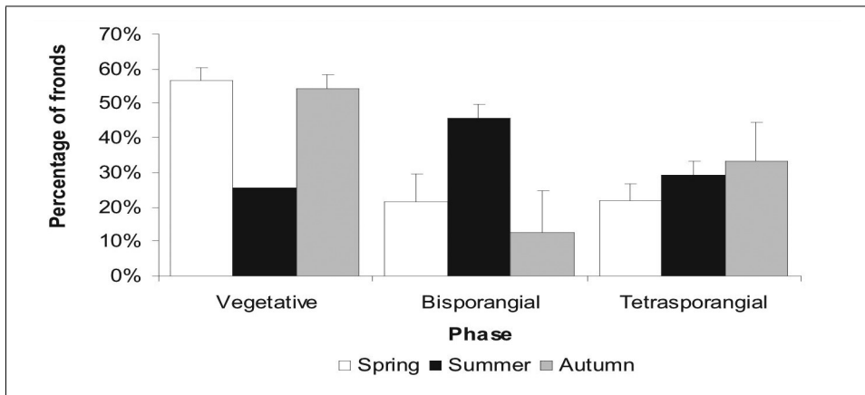
Fig. 4. Percentage of reproductive plants by season (mean + se: Spring and Autumn n = 3 , Summer n = 2 ). Vegetative fronds were dominant in spring, autumn and winter. Bisporangial and tetrasporangial phases occurred in less proportion, but were dominant during the summer months. Bars indicate standard errors.
