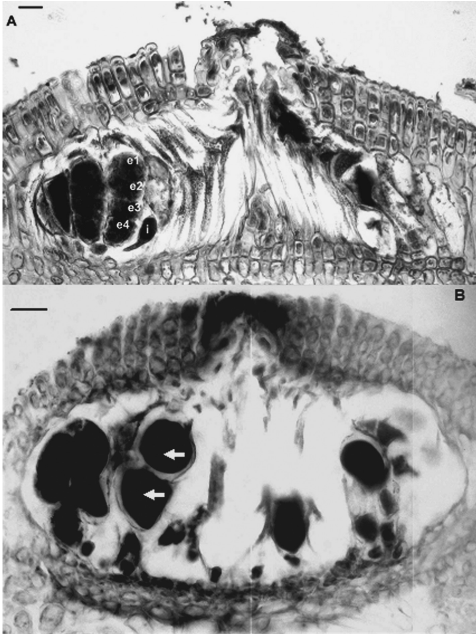
Fig. 3. Reproductive structures of A. beauvoisii from Isla Asunción. A. Tetrasporangial conceptacle showing mature tetrasporangium with spores (e1,e2,e3,e4) and immature tetrasporangium (i). B. Bisporangial conceptacle showing mature sporangium with bispores (white arrows). Bar scale 20 µm.
