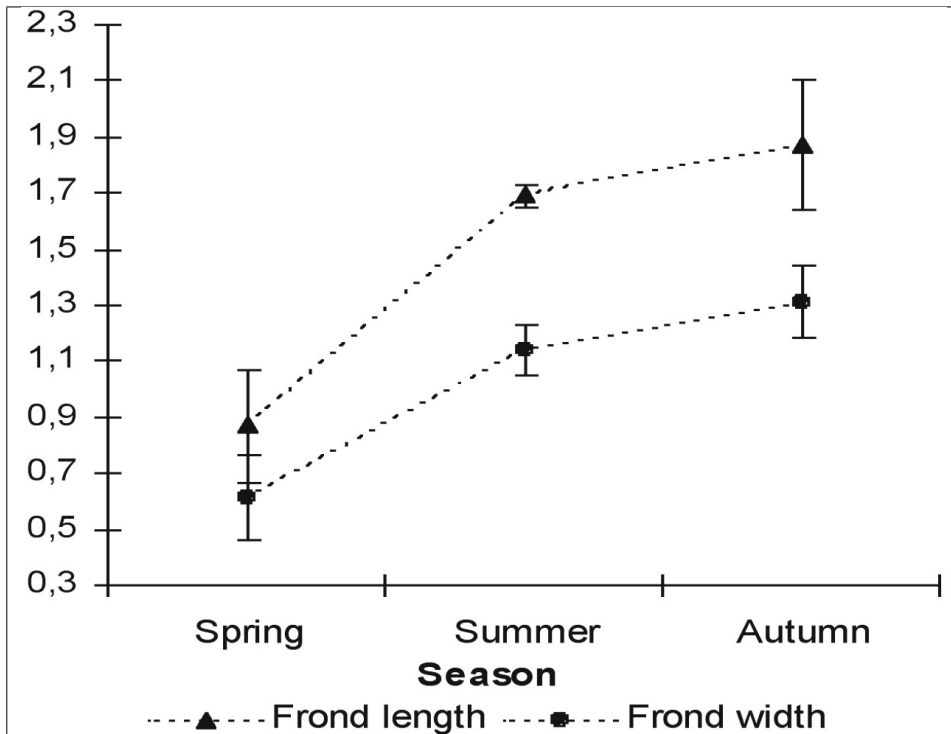
Fig. 1. Frond length and width (mean + se: Spring and Autumn n = 3 , Summer n = 2 ) showing a significant increment in size between spring and summer-autumn (length - F_{0.05, 2} = 7.14 , p < 0.05 and width - F_{0.05, 2} = 7.92 , p < 0.05 ). Bars indicate standard errors.
