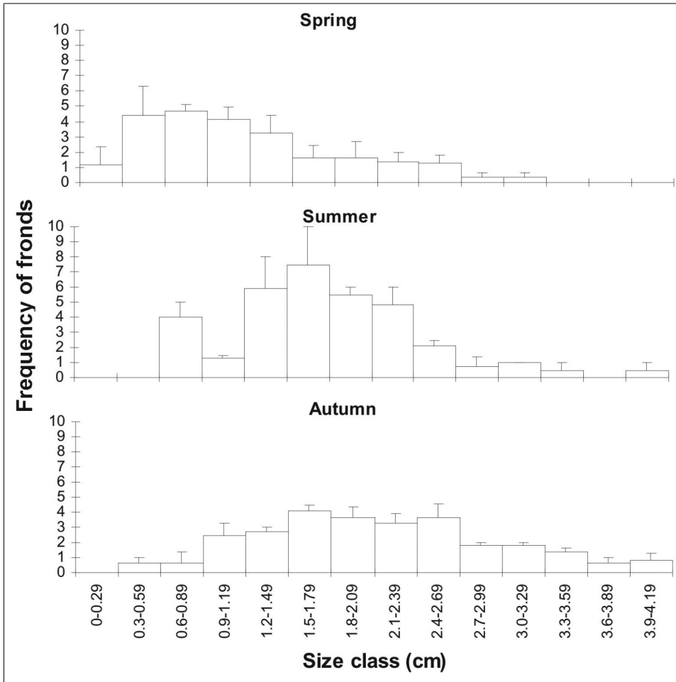
Fig. 2. Seasonal size-frequency histograms of fronds length, (mean + se: Spring and Autumn n = 3 , Summer n = 2 ), note that the frequency of small fronds (first size-class) is highest in spring than summer and autumn. Bars indicate standard errors.
