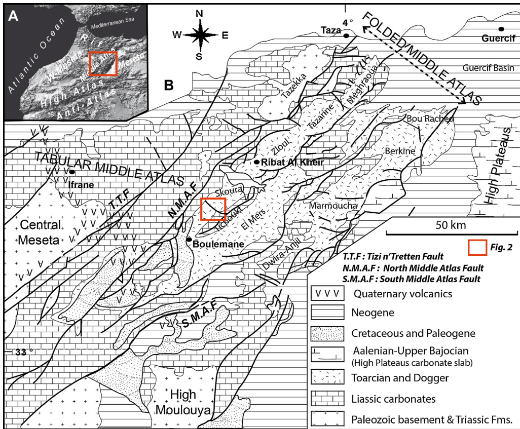
Fig. 1. A. Location of the Middle Atlas, B. Geological sketch map of the Middle Atlas and location of the study area (modified after Fedan et al., 1989).
