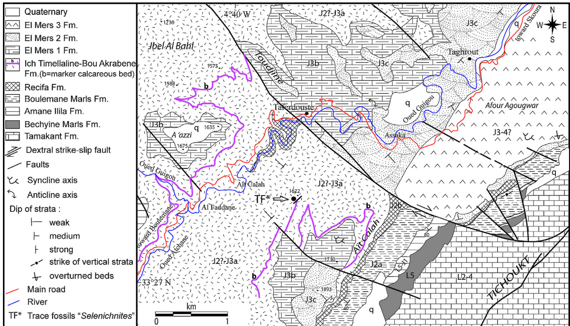
Fig. 2. Simplified geological map of the Skoura syncline (Middle Atlas, Morocco) after Charrière (1990), with additional field data.
