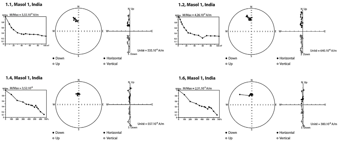
Fig. 6. Thermal and alternating field demagnetization for four samples from the Masol 1 Unit F (PPM1 block): change of the magnetization, stereographic projection, Zijderveld diagram.
