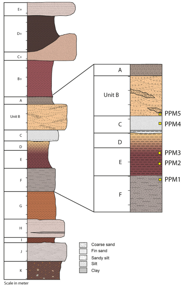
Fig. 3. Lithostratigraphy of the Masol 1 locality and location of the block-shaped samples.
