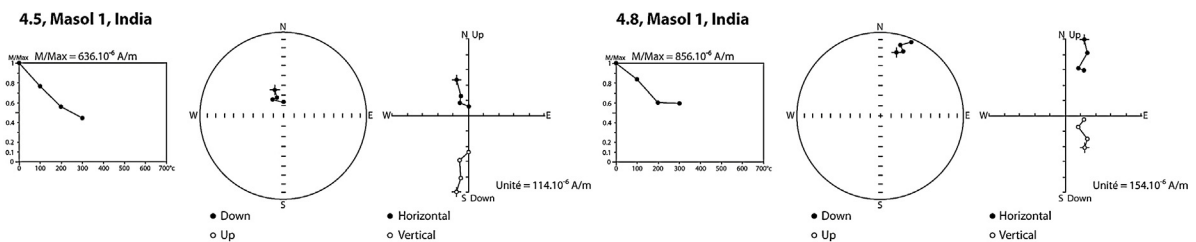
Fig. 8. Thermal demagnetization for the two Masol upper Unit E samples (PPM3 block): change of the magnetization, stereographic projection, Zijderveld diagram.
