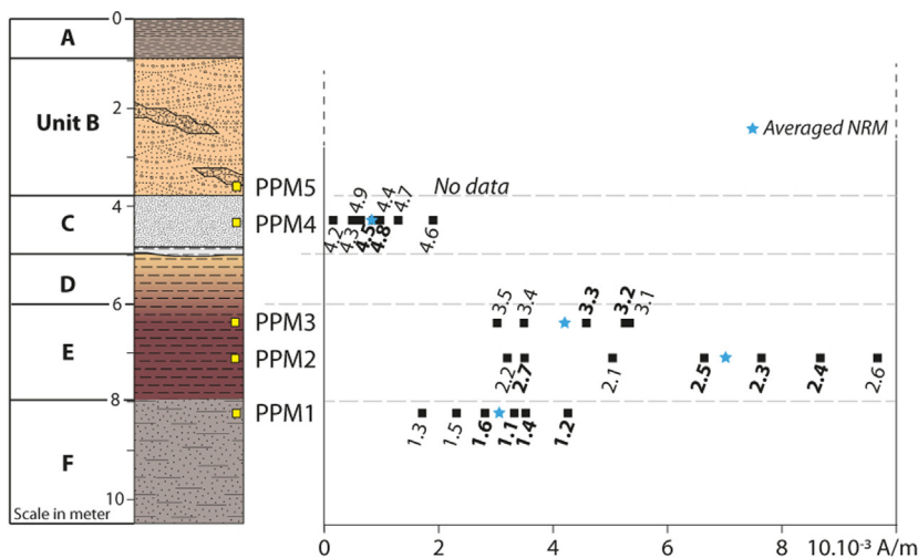
Fig. 4. Natural remanent magnetizations recorded in the cubic samples of the Masol 1 sediments. In bold, the selected samples for both demagnetizations (AF and thermal).
