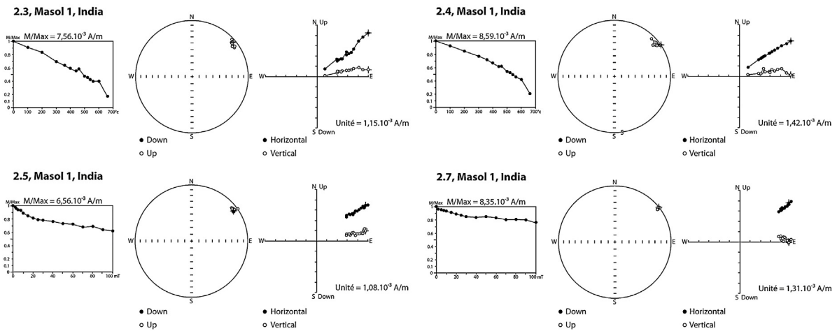
Fig. 7. Thermal and alternating field demagnetization for the four samples from the Masol lower unit E samples (PPM2 block): change of the magnetization, stereographic projection, Zijderveld diagram.
