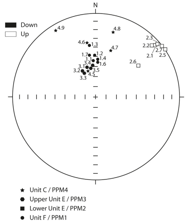
Fig. 5. Stereographic projection before the thermal and alternating field demagnetization of the whole cubic samples.
