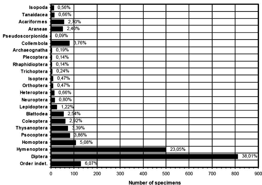
Fig. 2. Frequency distribution of arthropods found in Álava amber. The total number of arthropods found in the other localities is extremely low in comparison.
