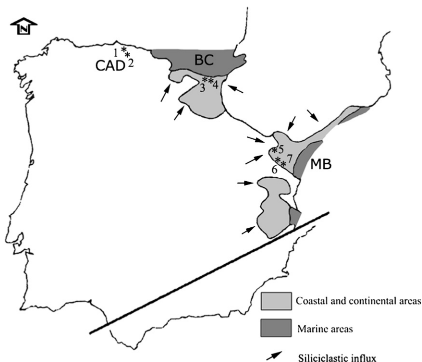
Fig. 1. Map of Spain showing the location of the Albian–Cenomanian basins and the Albian amber-bearing localities where palaeobiological inclusions are found. MB : Maestrat Basin, BCB : Basque Cantabrian Basin, CAD : Central Asturian Depression. 1. Pola de Siero, 2. El Caleyú, 3. Peñacerrada (= Peñacerrada II), 4. Moraza (= Peñacerrada I), 5. San Just, 6. Arroyo de la Pascueta, 7. La Hoya. Early–Middle Albian Iberian Plate reconstruction after [45].
