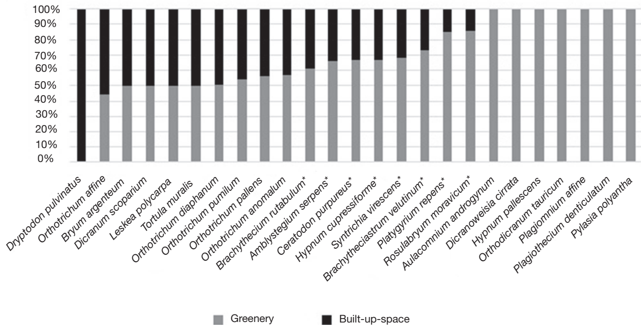
FIG. 2. — Comparison of the percentage of incidence of individual bryophyte species on trunks of alien host trees situated in complexes of urban greenery and urban buildings. Key: Species for which statistical significance ( p < 0.05 ) was found in preferences to occur more frequently in one of the land-use complexes are marked with an asterisk . Tests were not performed in cases in which one of the components (population in greenery or built-up space) was equal to zero.
