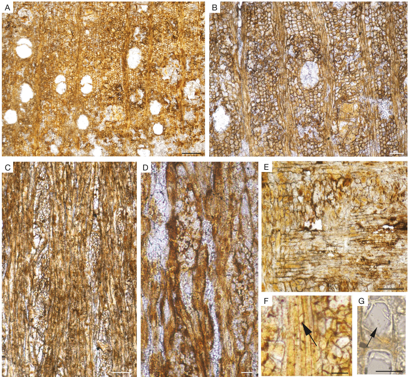
FIG. 14. — Celtis cf. integrifolia , Twf 17812: A, B , Tr, mostly solitary vessels with confluent or seemingly banded axial parenchyma; C, D , Tg, wide heterocellular rays; E , Rd, heterocellular rays; F , Tr., Prismatic crystal in ray-cell ( arrow ); G , Tg, detail of crystal in ray cells. Scale bars: A, 200 \mu m; B, C, E, 100 \mu m; F, 50 \mu m; D, G, 20 \mu m. Photographs: M.-C. Jolly-Saad.
