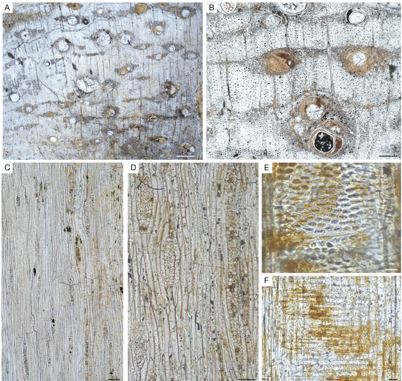
FIG. 43. — Peltophorum sp. (Fabaceae Lindl.), Twf 17968: A, B , Tr, wood diffuse porous, Parenchyma is vasicentric enclosing vessels or group of vessels to form aliform, winged aliform to confluent and marginal bands composed of 2-3 cells; C, D , Tg, rays 1-3 seriate; E , intervessel-pits vestured; F , Rd, heterocellular rays. Scale bars: A, 200 µm; B, C, 100 µm; D, 50 µm; E, 10 µm; F, 20 µm. Photographs: M.-C. Jolly-Saad.
