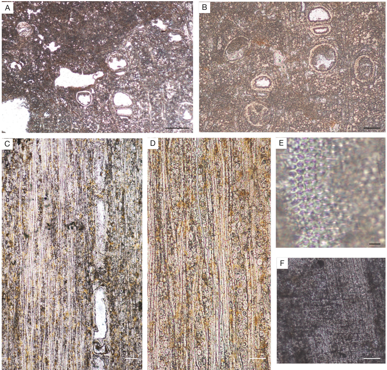
FIG. 4. — Combretaceae/Fabaceae gen. and sp. indet. 1, Twf 17873: A, B , Trs, diffuse vessels and seemingly and wavy banded parenchyma arrangement; C, D , Tg, rays 1-2 (3) seriate; E , Tg, vestured intervessel-pits; F , Rd, heterocellular rays. Scale bars: A, 200 \mu m; B, C, 100 \mu m; D-F, 50 \mu m; E, 10 \mu m. Photographs: M.-C. Jolly-Saad.
