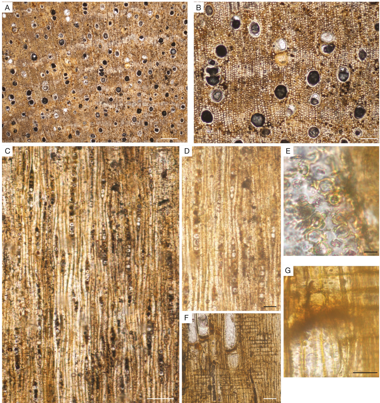
FIG. 49. — Sapindaceae gen. and sp. indet., Twf 17966: A, B , Tr, vessels diffuse, axial parenchyma scanty paratracheal and in marginal bands; C, D , Tg, rays uniseriate or locally biseriate; E , Tg, intervessel pits; F, G , Rd, heterocellular rays; G , detail of radiovascular pits. Scale bars: A, 200 µm; B, C, 100 µm; D, F, 50 µm; E, 10 µm; G, 20 µm. Photographs: M.-C. Jolly-Saad.
