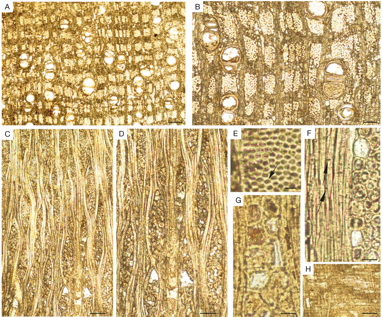
FIG. 6. — Entandrophragma sp. 1 (Meliaceae Juss.), Twf 17913: A, B , Tr, vessels solitary or in radial multiple, axial parenchyma with wavy band arrangement; C , Tg, 1-5 seriate rays; D , Tg, detail of rays with rays marginal square and upright cells; E , Tg, fibres with septae; F , Tg, minute and not vested minute intervessel-pits; G , Rd, heterocellular rays; H , Rd, crystal in ray cell (arrow). Scale bars: A, 200 \mu m; B, C, 100 \mu m; D, F, H, 50 \mu m; E, 25 \mu m; G, 5 \mu m. Photographs: M.-C. Jolly-Saad.
