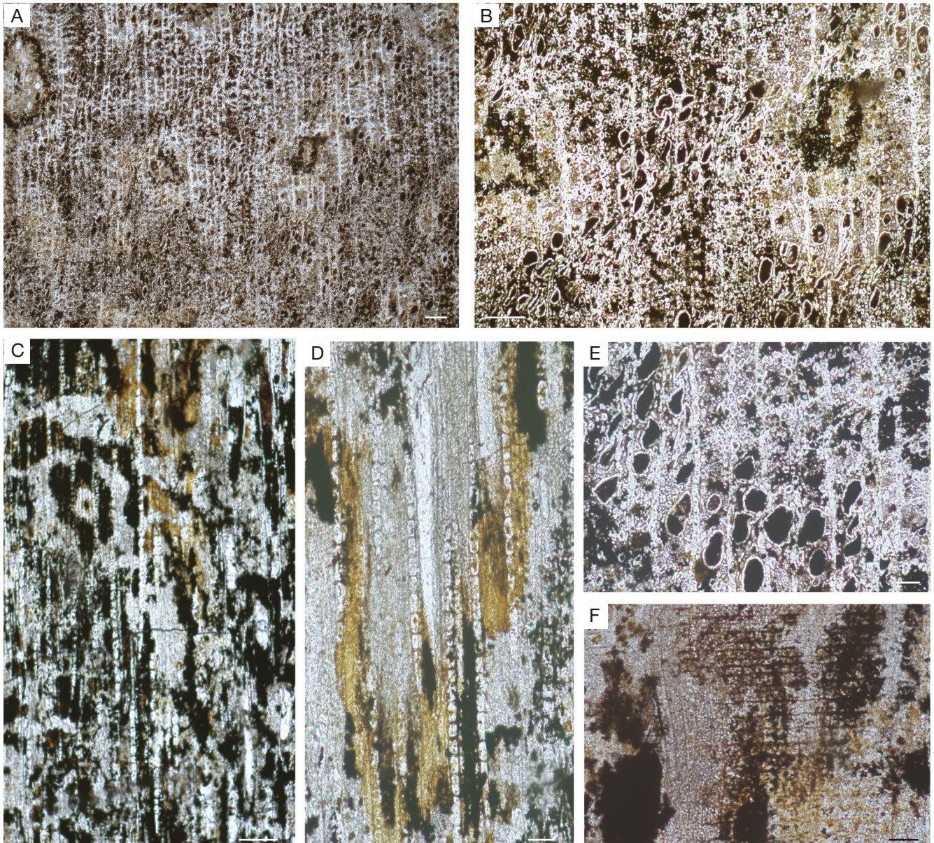
FIG. 48. — Sapotaceae gen. and sp. indet., Twf 17636: A, B , Tr, wood diffuse porous with a dendritic arrangement; axial parenchyma diffuse-in-aggregate; E , Tr, detail transversal section with vessel repartition and parenchyma cells; C, D , Tg, rays 1-2 seriate with square and upright cells; F , Rd, heterocellular rays. Scale bars: A-C, 100 \mu m; D-F, 50 \mu m. Photographs: M.-C. Jolly-Saad.
