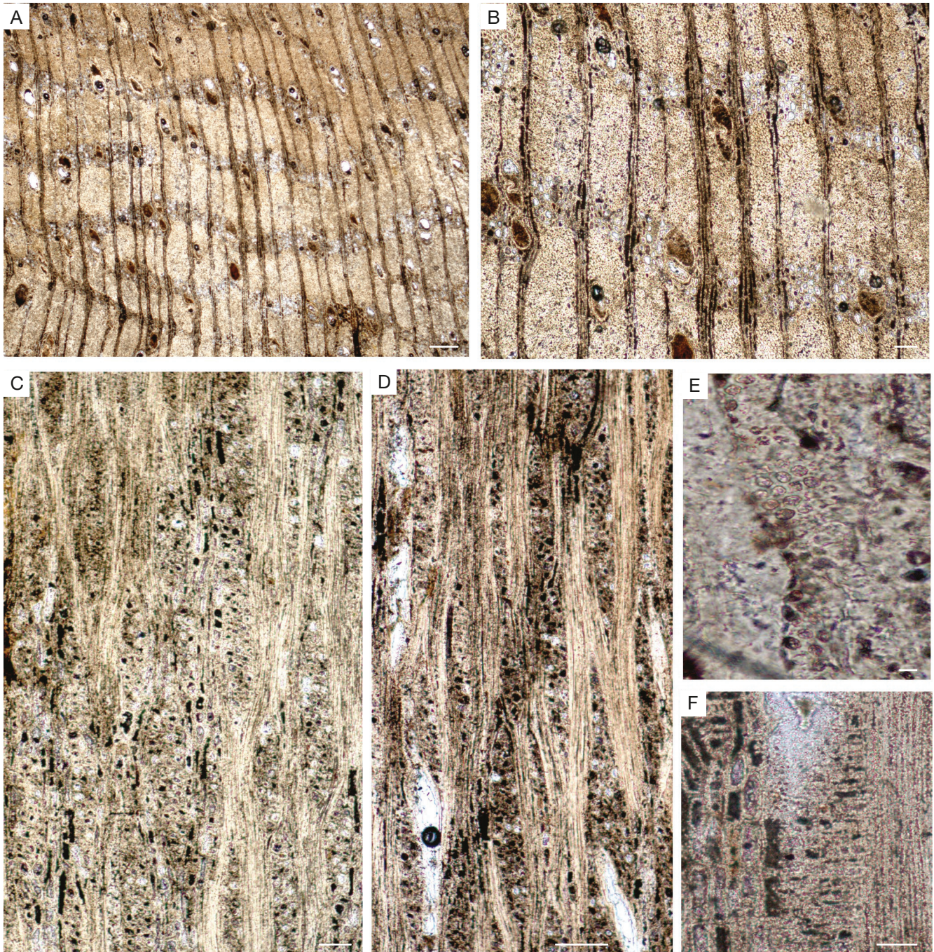
FIG. 9. — Terminalia sp. 2, Nfw001: A, B , Trs, vessels located in short wavy bands of parenchyma; C, D , Tgs, heterocellular rays; E , Tg, vestured intervessel-pits; F , Rds, heterocellular rays. Scale bars: A, 200 \mu m; B, C, 100 \mu m; D, F, 50 \mu m; E, 5 \mu m. Photographs: M.-C. Jolly-Saad.
