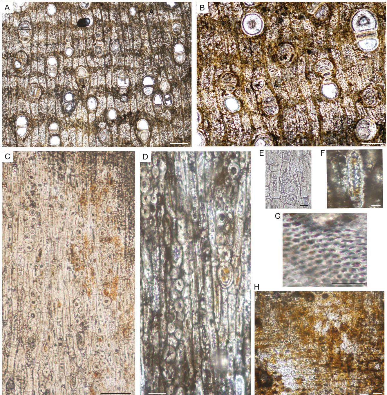
FIG. 3. — Terminalia sp. 1 (Combretaceae), Twf 17918: A , Transverse section ( Tr ), solitary vessels or in radial multiple and banded or seemingly banded parenchyma; B , Tr , detail of axial parenchyma C , Tangential section ( Tg ), 1-3 seriate heterocellular rays; D , Tgs , detail of rays with crystal in enlarged cells; E , Tg , vestured intervessel-pits; F , Tg , druses in parenchyma cell; H , Radial section ( Rd ), heterocellular rays. Scale bars: A, 200 µm; B, 100 µm; D, 50 µm; E, F, 10 µm; G, H, 20 µm. Photographs: M.-C. Jolly-Saad.
