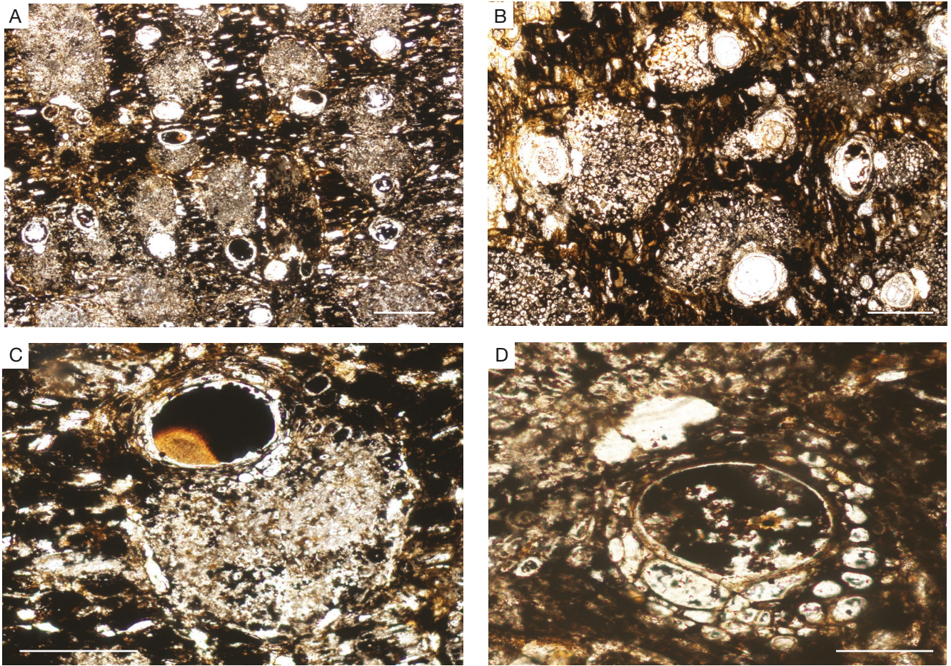
FIG. 36. — Borassus sp. 1 (Arecaceae Bercht. & J.Presl.), Twf 17830: A-D , Tr, fibrovascular bundles with one vessel. Scale bars: A, D, 200 \mu m; B, 100 \mu m; C, 90 \mu m. Photographs: M.-C. Jolly-Saad.
