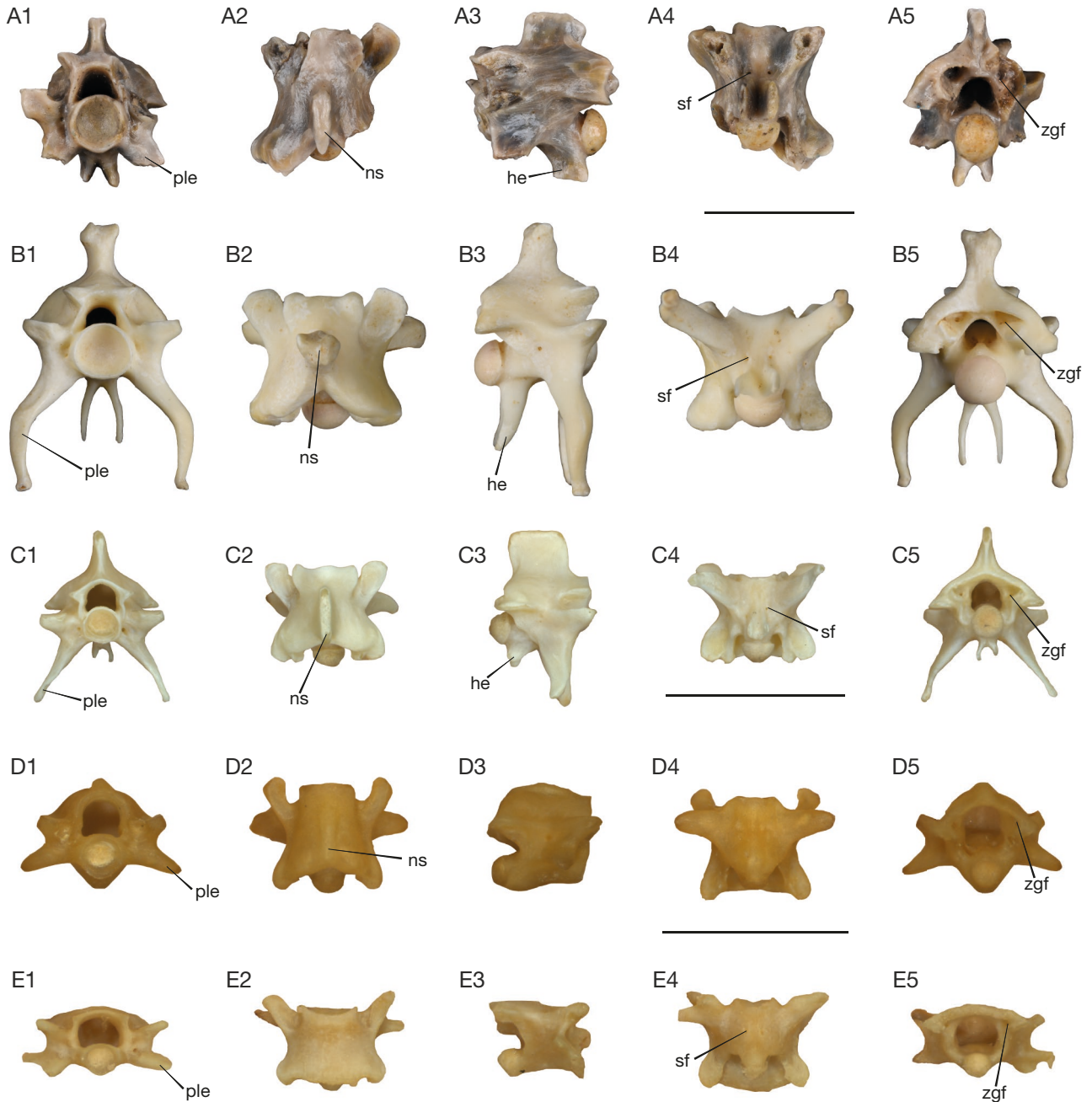
FIG. 7. — Comparison of VPPLT-1740 post cloacal vertebrae with extant aletinophidians: A , VPPLT-1740 specimen; B , Boa cf. constrictor Linnaeus, 1758, VPPLT-uncatalogued specimen; C , Tropidophis melanurus (Schlegel, 1837), UF-H-52001; D , Anilius scytale Linnaeus, 1758, UF-H-52001; E , Cylindrophis ruffus Laurenti, 1768, UF-H-52673. Views: 1 , anterior; 2 , dorsal; 3 , lateral; 4 , ventral, 5 , posterior views. Scale bars: A, B, 10 mm; C, 5 mm; D, E, 3 mm.
