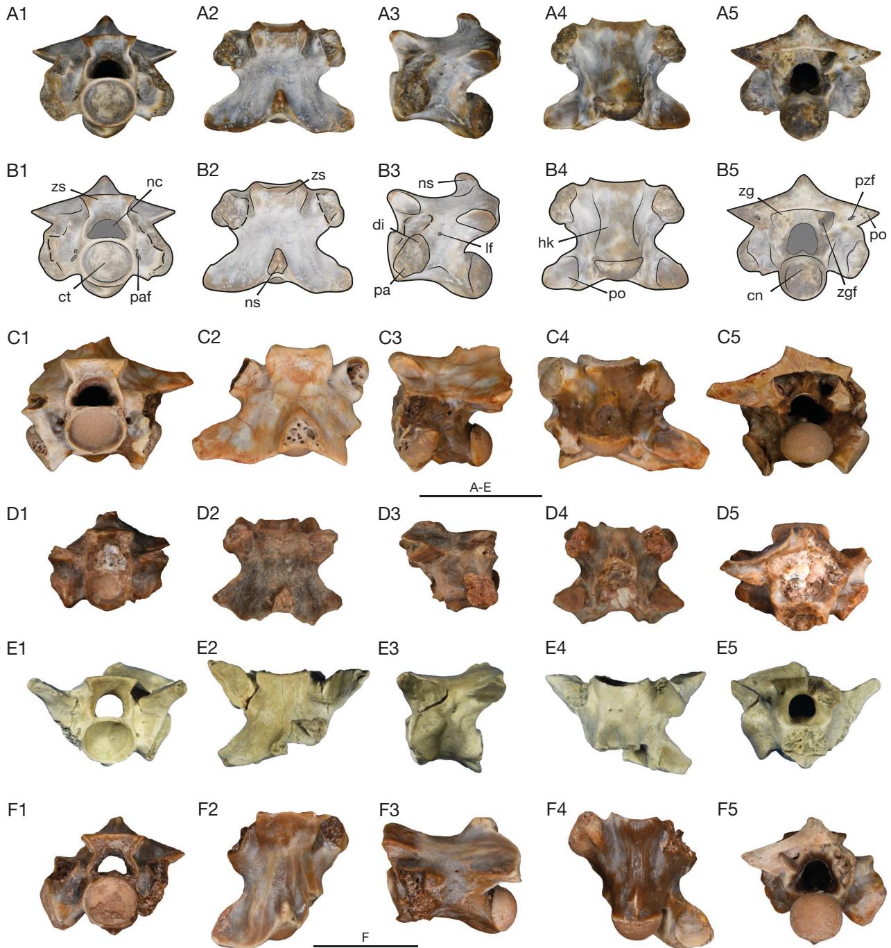
FIG. 6. — Colombophis spinosus Hsiou, Albino & Ferigolo, 2010 from the Tatacoa Desert: A, B , VPPLT-1728; C , VPPLT-0798; D , VPPLT-1093; E , VPPLT-1741; F , VPPLT-1534. Views: 1 , anterior; 2 , dorsal; 3 , lateral; 4 , ventral, 5 , posterior views. Scale bars: 10 mm.
