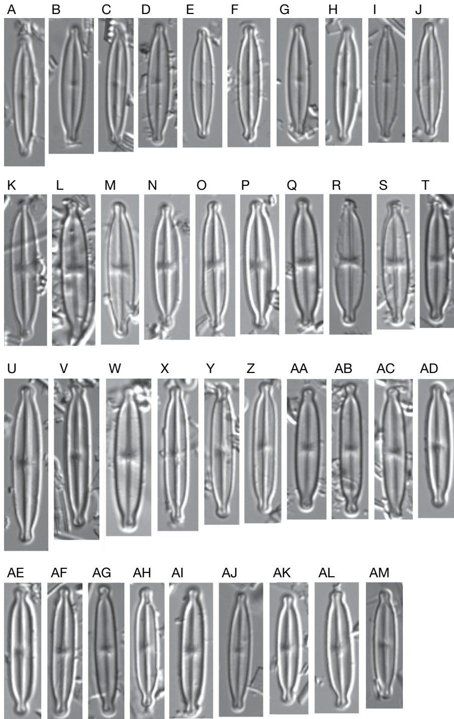
FIG. 3. — Light micrograph diminution series of Kobayasiella Lange-Bertalot species: A–J , Kobayasiella tursujuquensis sp. nov.; K–T , Kobayasiella pseudostauroon (Lange-Bertalot) Lange-Bertalot. Scale bar: 10 \mu m.
