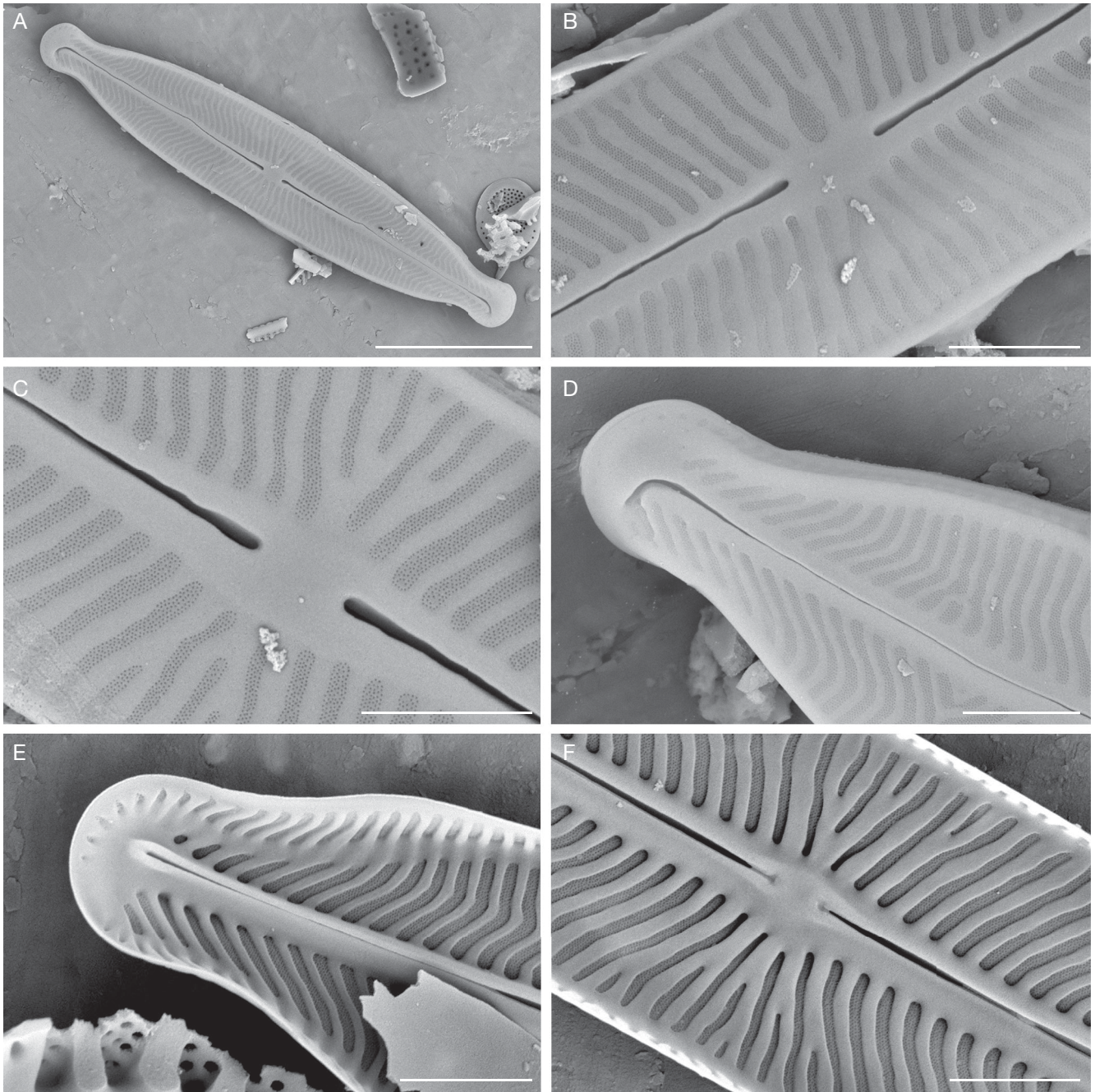
FIG. 7. — SEM images of Kobayasiella tursujuqensis sp. nov.: A , external view of the complete valve; B, C , external views of the central area showing the multi-seriate poroid covers between irregularly formed virgae; D , external view of the valve apex showing a bent proximal fissure opening into an irregular surface depression; E , internal valve view of the apex. Helictoglossa expanded onto a highline apex. Areolae interrupted around the apex; F , internal view of the axial and central areas with T-shaped proximal fissures with a central surface depression between the fissures. Scale bars: A, 5 \mu m; B-F, 1 \mu m.
